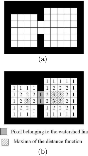
Fig. 2. (a) Binary image. (b) Associated distance function.
