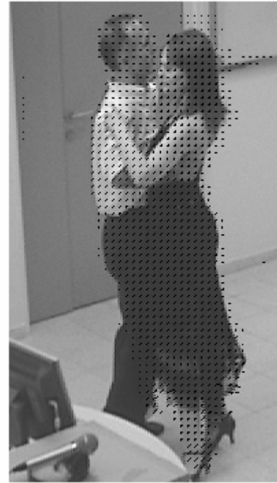
Our Method
