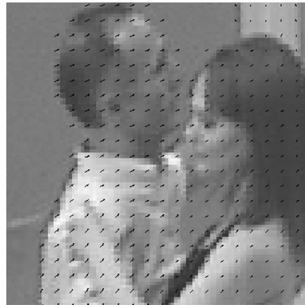
Our Method
